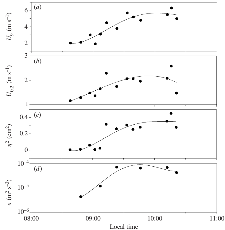
FIGURE 23. (a) Wind speed at 9 m above the water surface (150 s average), (b) wind speed at 20 cm above the water surface (75 s) average, (c) wave height variance (75 s average), (d) turbulent kinetic energy dissipation.
