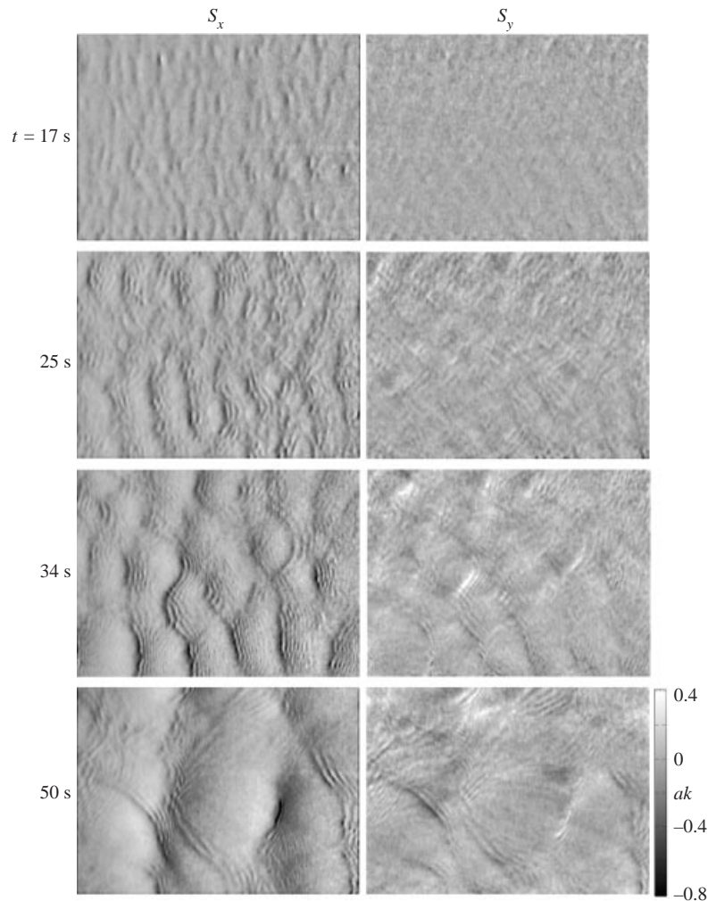
FIGURE 3. Along-wind slope, S_x , and cross-wind slope, S_y , of the surface wave field at t = 17, 25, 34 and 50 s for a final wind speed of 5 \text{ m s}^{-1} , at a fetch of 10.72 m. Image size is 36.8 cm by 27 cm. The wind is blowing from left to right.
