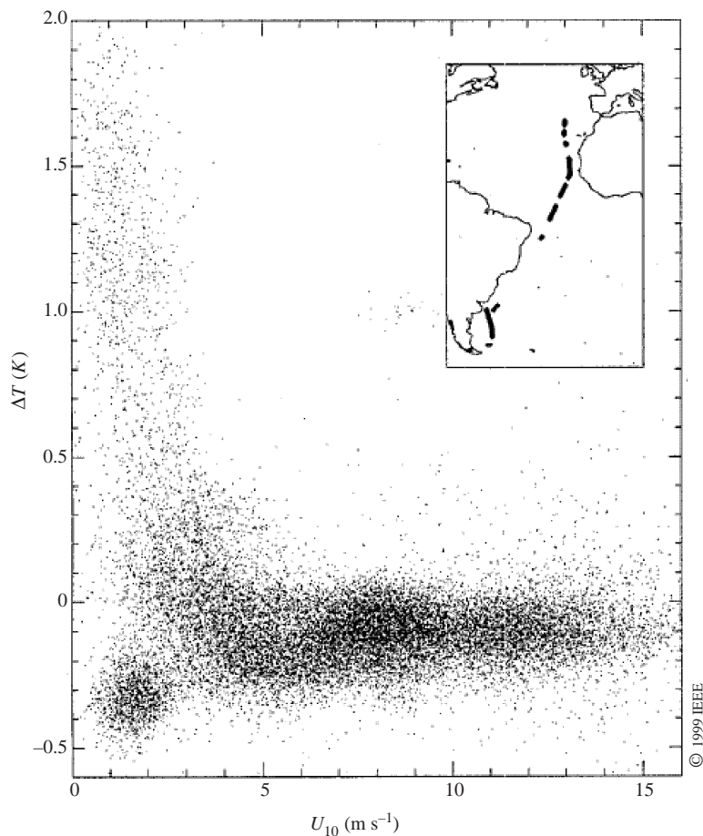
FIGURE 26. 10 m wind speed plotted against \Delta T for the entire Atlantic AMT-3 data set (from Donlon et al. 1999).
