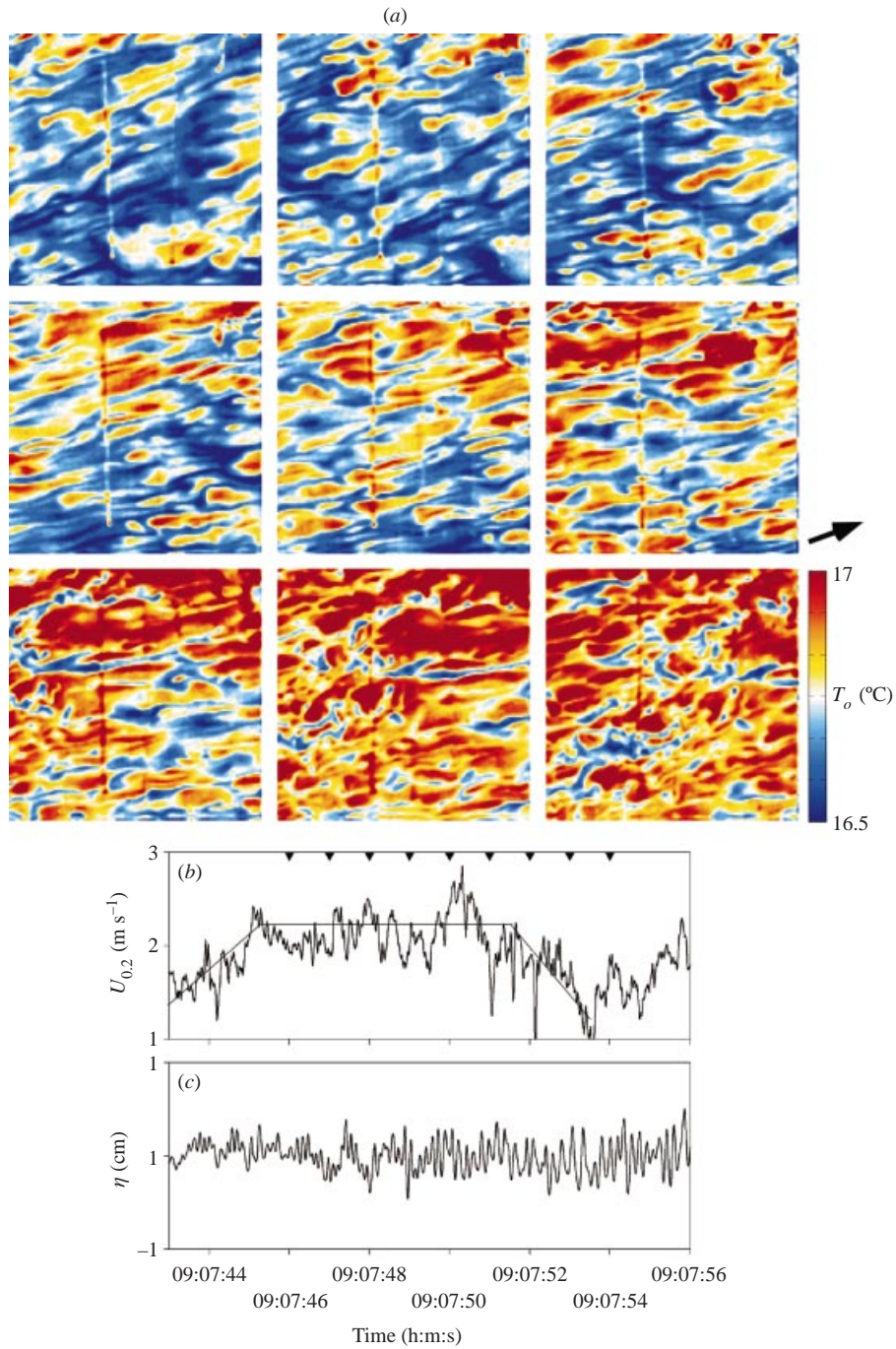
FIGURE 24. (a) Surface temperature images taken on 4 April 2000. Image size is 53.35 \text{ cm} \times 53.35 \text{ cm} . Times shown are t = 09:07:46 to 09:07:54 a.m. at 1 s intervals (left to right, top to bottom). The wind direction is given by the arrow. Note the evolution of the surface temperature as the surface is disrupted by the Langmuir circulations. Note also that the average surface temperature increases. (b) Time series of the wind speed and (c) wave heights. Note the variability in the wind speed and the growth of the wave amplitude. The inverted triangles denote the times of the IR images shown in (a).
